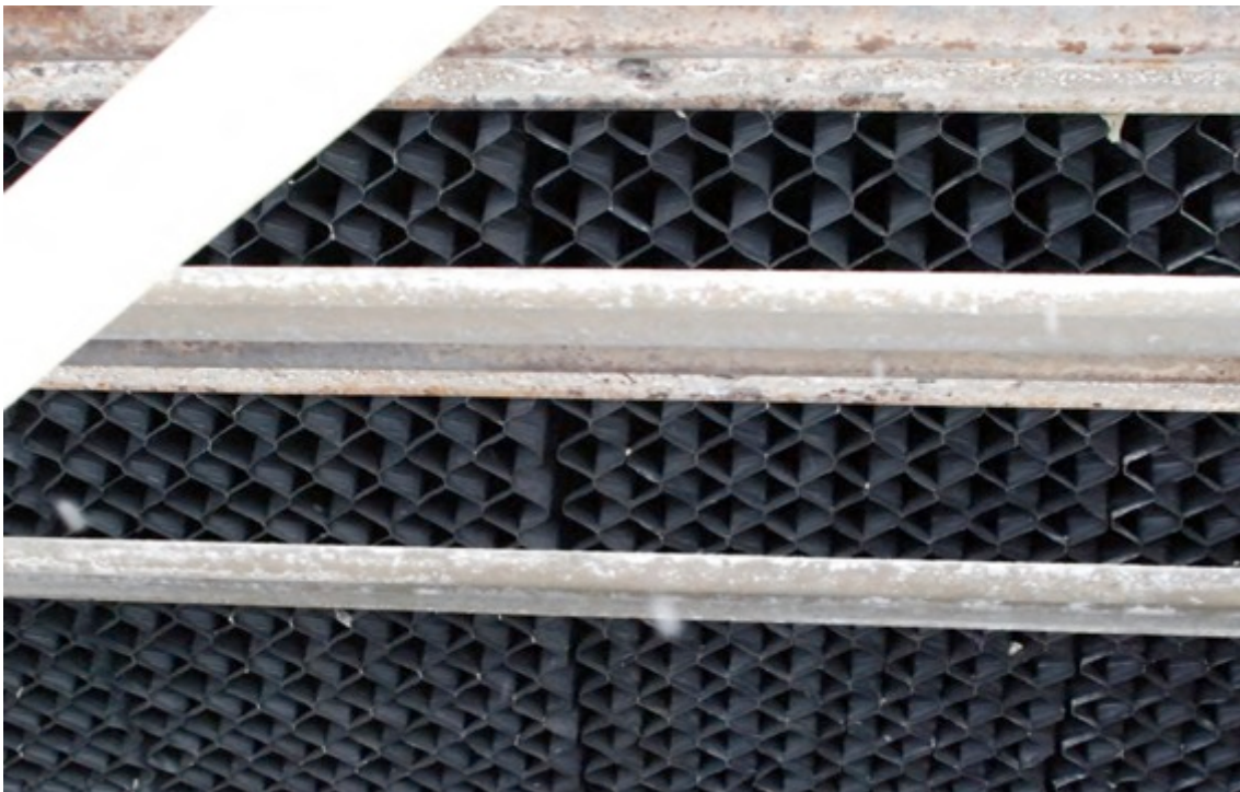
Cooling tower media from 16 year old phase one test facility after two cooling seasons on ProMoss™
